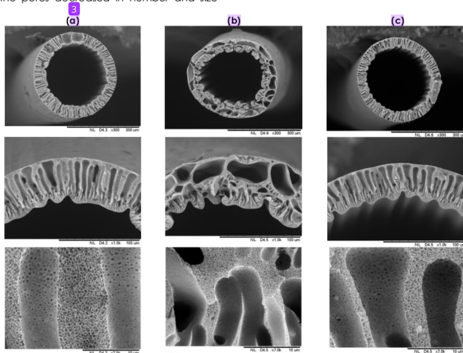
Figure 2 The cross sectional SEM images of (a) PES/CA, (b) PES/CA/ZA and (c) PES/CA/IZC
