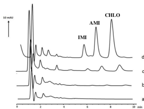
Figure 9. Chromatograms of TCAs in lake water, a. unspiked, b. spiked at 10 \mu\text{g.L}^{-1} , c. spiked at 50 \mu\text{g.L}^{-1} , d. spiked at 500 \mu\text{g.L}^{-1}
