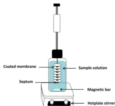
Figure 1. Set-up of thin-film microextraction (TFME) technique
