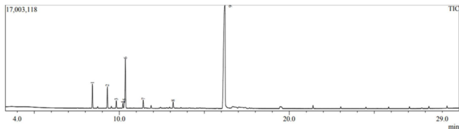
Figure 2. Total Ionic Chromatogram of Laja Gowah Oil
