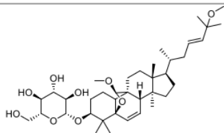
Goyaglycoside-c
