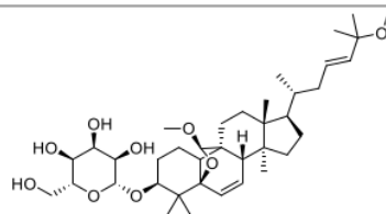
Goyaglycoside-d
