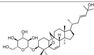
Momordicoside I
