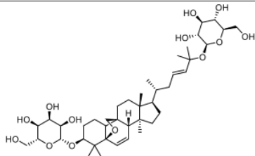
Goyaglycoside-e
