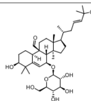
Momordicoside K
