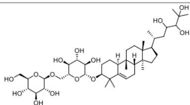
Momordicoside C
