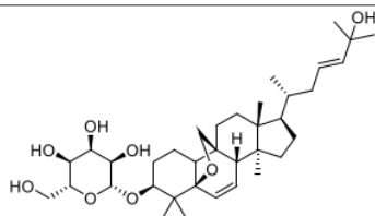
Momordicoside F2
