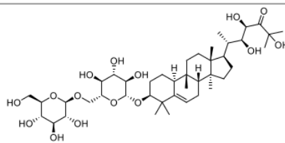
Goyaglycoside-h
