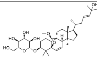
Goyaglycoside-b
