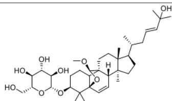
2 Goyaglycoside-a
