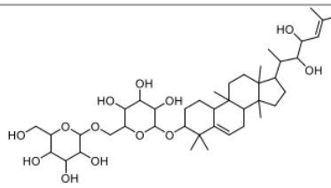
Momordicoside D
