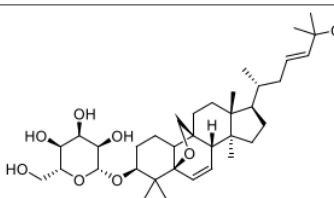
Momordicoside G
