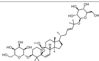
Goyaglycoside-g
