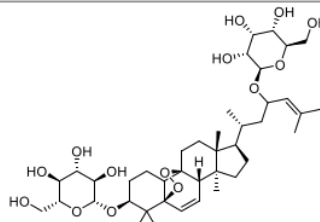
Goyaglycoside-f
