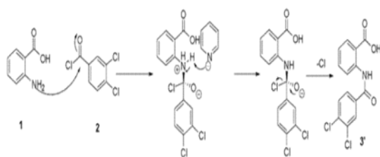
Fig. 5: Reaction mechanism between anthranilic acid (1) and 3,4-dichlorobenzoyl chloride to form 2-(3,4-dichlorobenzamido)benzoic acid (3')
