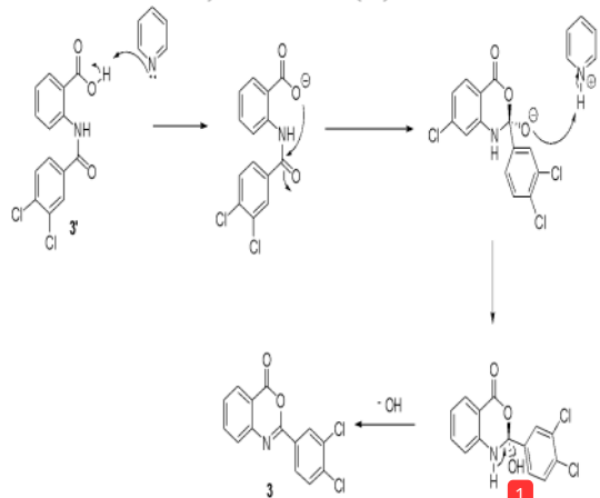
Fig. 6 : Reaction mechanism of the formation of 2-(3,4-dichlorophenyl)-4H-benzo[d][1,3]oxazin-4-one (3)
